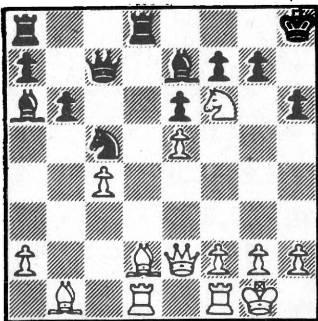
177 After 19...Kh8
